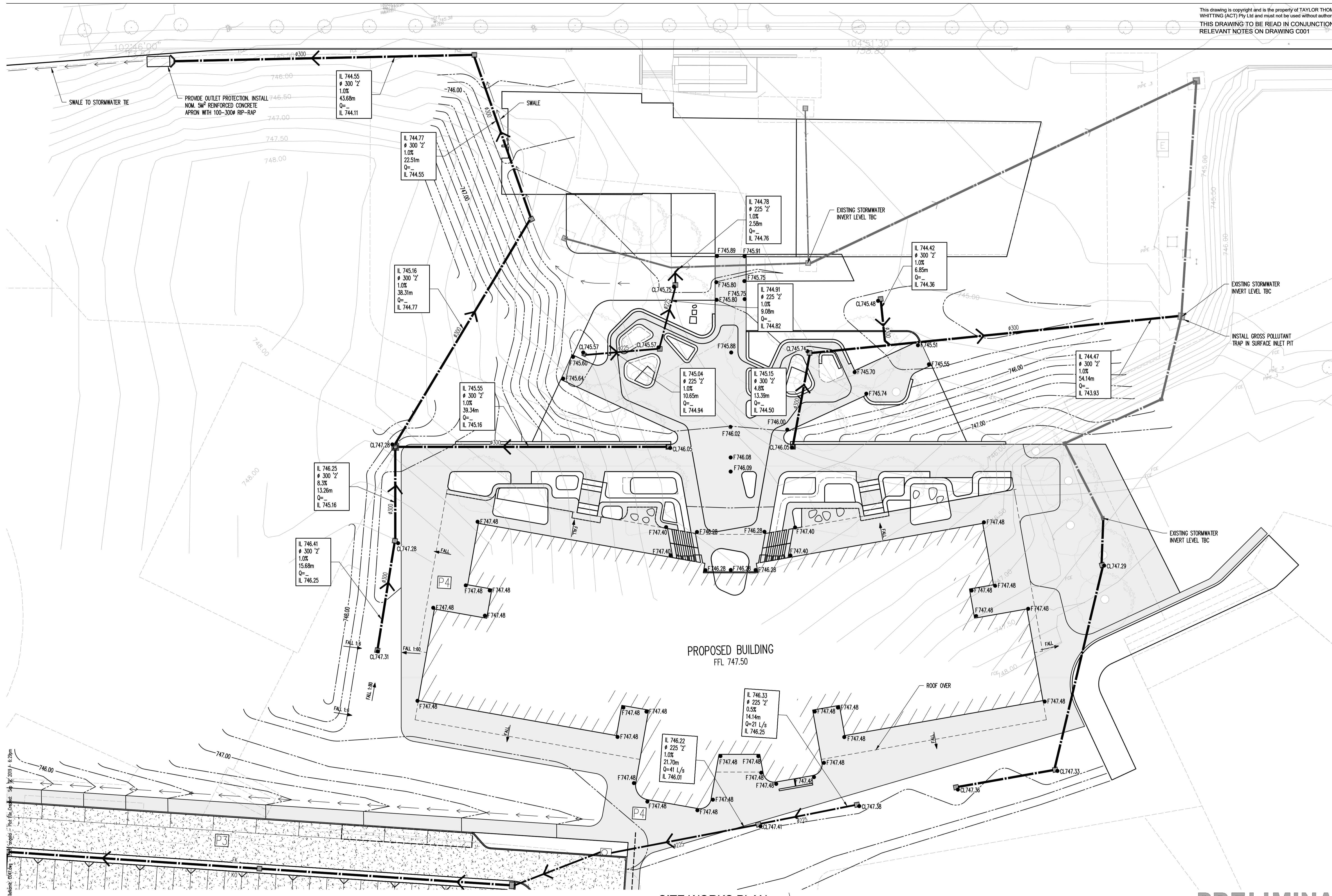
SITE WORKS PLAN SCALE 1: 250
